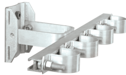
Aluminum stand off bracket with H-Bar and conduit straps SP-6060 SP-6049
