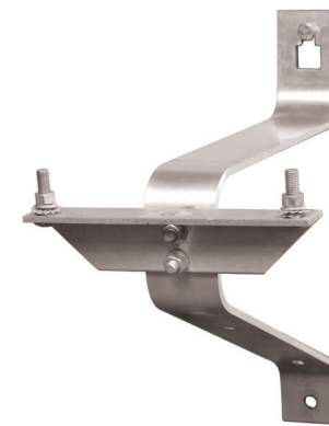
Aluminum standoff cutout and arrestor mount, standoff 17" from pole
