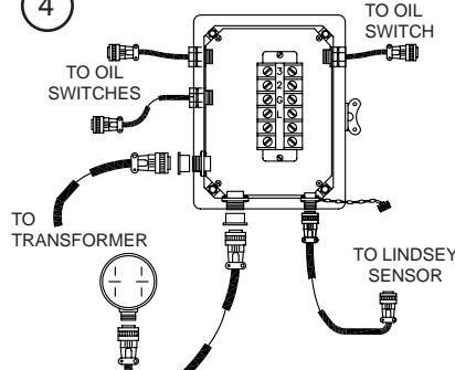
TYPICAL VAR CONTROL
