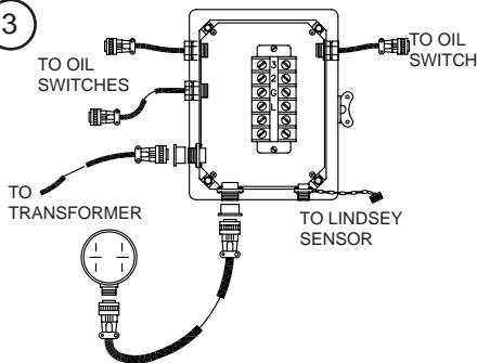
TYPICAL TIME & TEMP CONTROL
