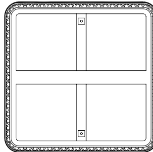
AP-7237 Cast Alum Sign Frame for 24" x 24" Sign
