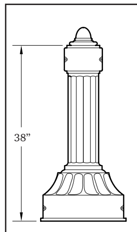
AP-0603 Le Grande Non-illuminated Bottom Opening 17" Max.
