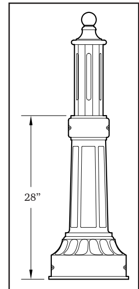
AP-0601 Country Club Illuminated Bottom Opening 11" Max.
